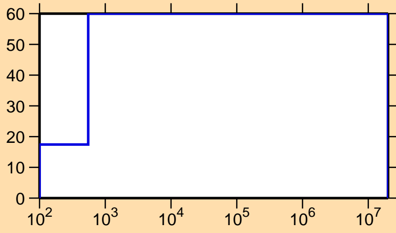
\Delta\sigma/\sigma vs. E for ^{176}\text{Pt}(n,\gamma)
