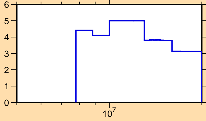
\Delta\sigma/\sigma vs. E for ^{177}\text{Pt}(n,\text{tot.})
