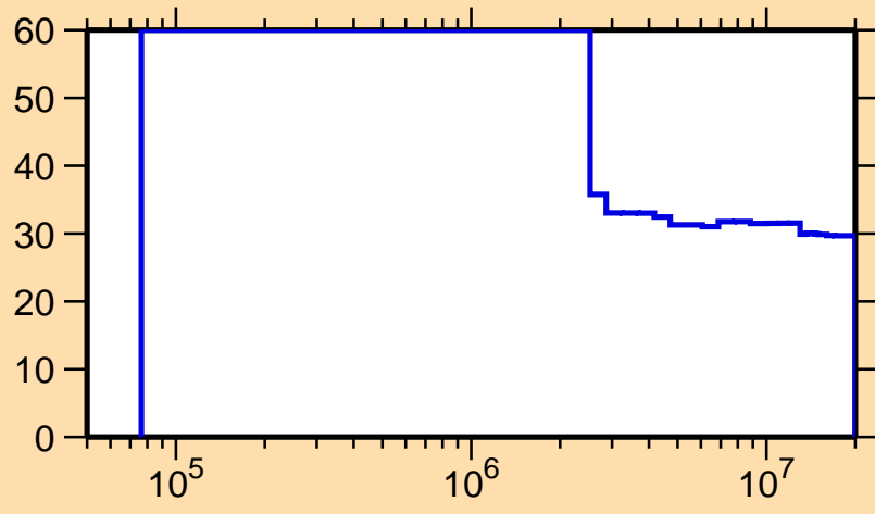
\Delta\sigma/\sigma vs. E for ^{177}\text{Pt}(n,n_1)
