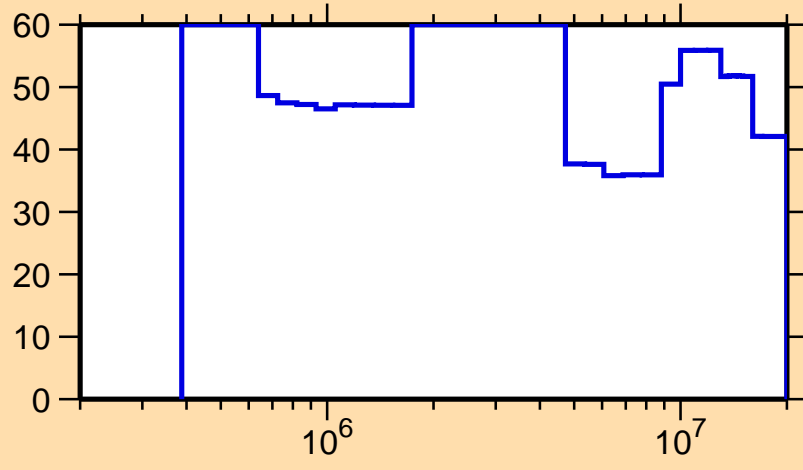
\Delta\sigma/\sigma vs. E for ^{177}\text{Pt}(n,n\text{cont.})
