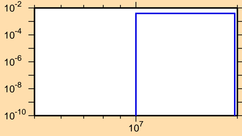
\sigma vs. E for ^{177}\text{Pt}(n,2n\alpha)
