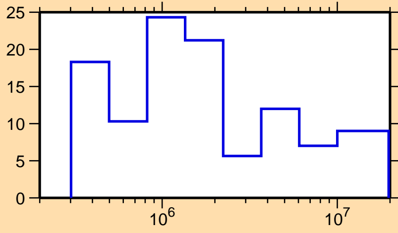
\Delta\sigma/\sigma vs. E for ^{177}\text{Pt}(n, el.)
