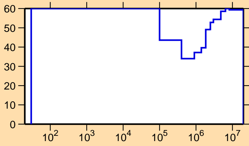
\Delta\sigma/\sigma vs. E for ^{177}\text{Pt}(n,\gamma)
