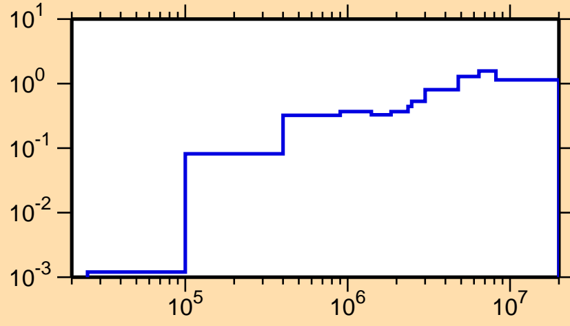
\sigma vs. E for ^{177}\text{Pt}(n,\text{inel.})
