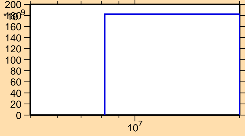
\sigma vs. E for ^{177}\text{Pt}(n,\text{pt})
