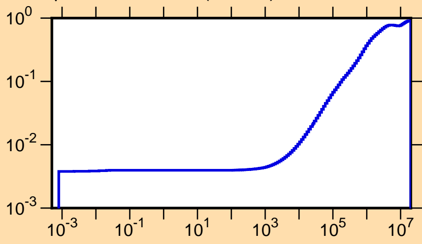
\mu vs. E for ^{178}\text{Pt}(\text{mt251})
