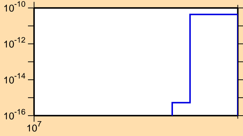
\sigma vs. E for ^{178}\text{Pt}(n,nt)
