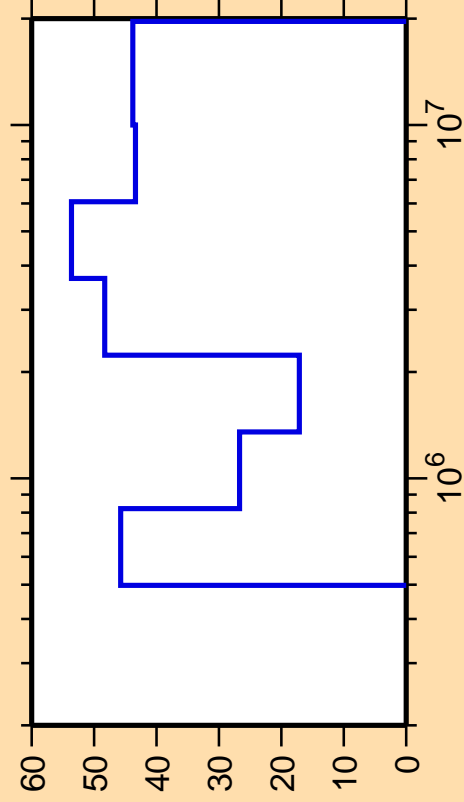
\Delta\sigma/\sigma vs. E for ^{178}\text{Pt}(n,n_4)
