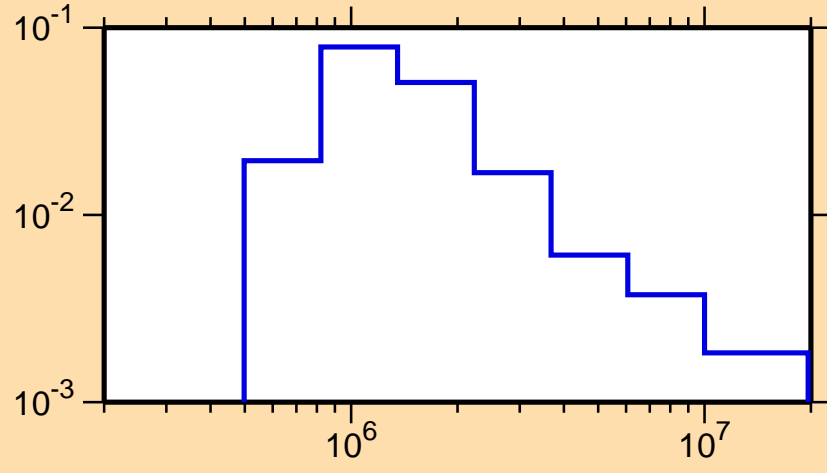
\sigma vs. E for ^{178}\text{Pt}(n,n_4)
