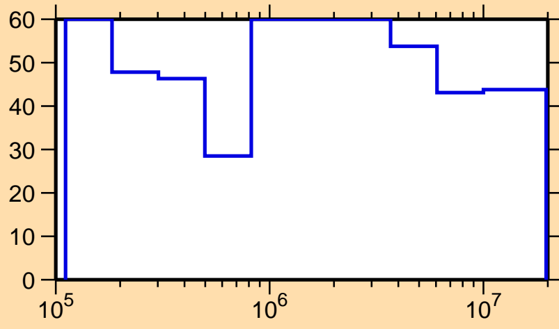
\Delta\sigma/\sigma vs. E for ^{178}\text{Pt}(n,n_1)
