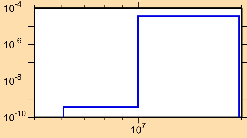
\sigma vs. E for ^{178}\text{Pt}(\text{mt } 45)
