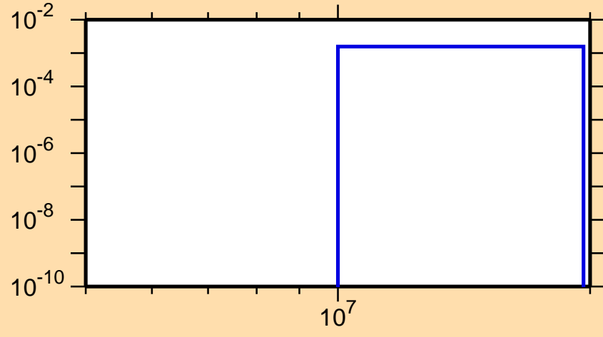
\sigma vs. E for ^{178}\text{Pt}(n,2n\alpha)
