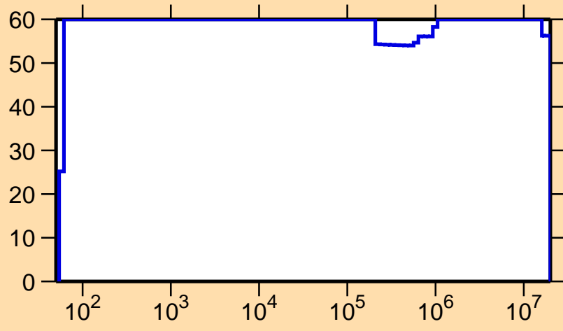
\Delta\sigma/\sigma vs. E for ^{179}\text{Pt}(n,p)
