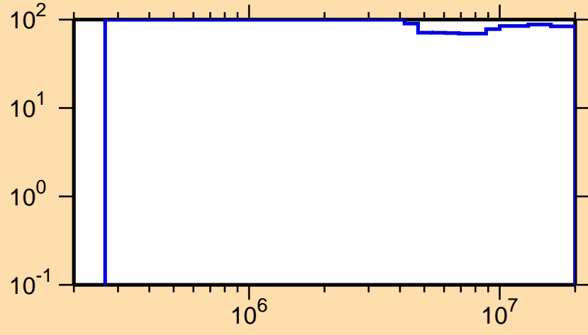
\Delta\sigma/\sigma vs. E for ^{179}\text{Pt}(n,ncont.)
