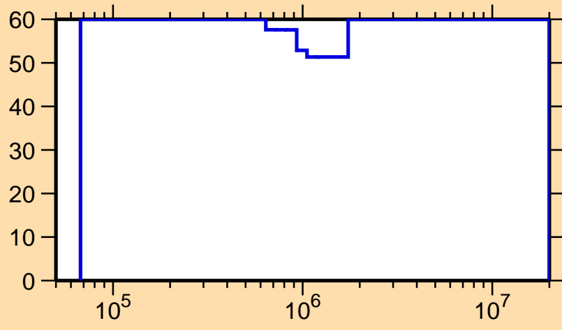
\Delta\sigma/\sigma vs. E for ^{179}\text{Pt}(n,n_1)
