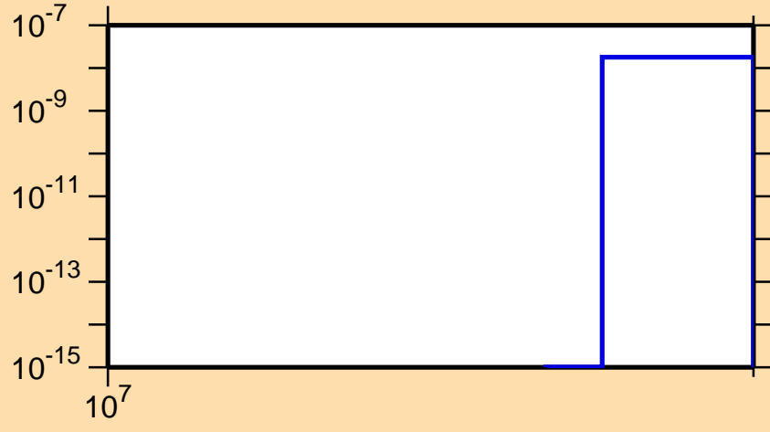
\sigma vs. E for ^{179}\text{Pt}(n,3n\alpha)
