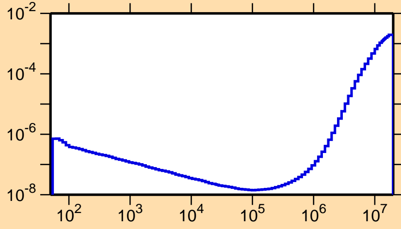
\sigma vs. E for ^{179}\text{Pt}(n,p\alpha)
