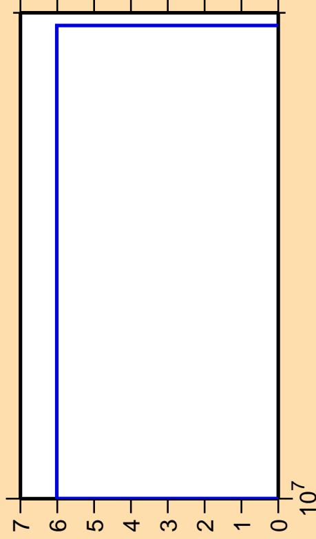
\Delta\sigma/\sigma vs. E for ^{179}\text{Pt}(n,nt)
