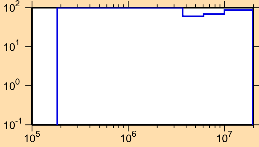
\Delta\sigma/\sigma vs. E for ^{179}\text{Pt}(n,n\text{cont.})
