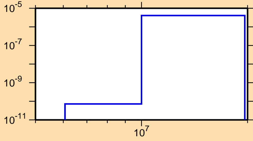
\sigma vs. E for ^{179}\text{Pt}(n,\text{He3})
