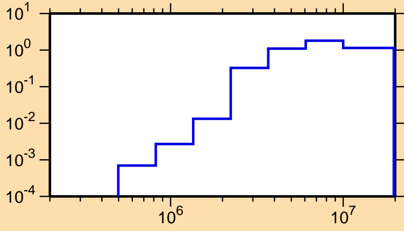
\sigma vs. E for ^{179}\text{Pt}(n,n\text{cont.})
