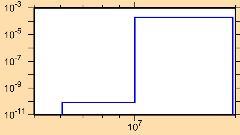
\sigma vs. E for ^{179}\text{Pt}(n,t)
