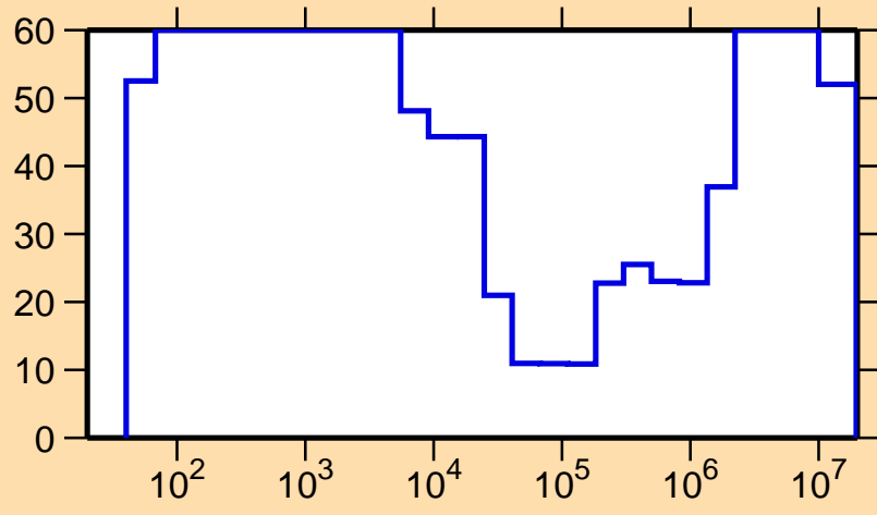
\Delta\sigma/\sigma vs. E for ^{179}\text{Pt}(n,\gamma)
