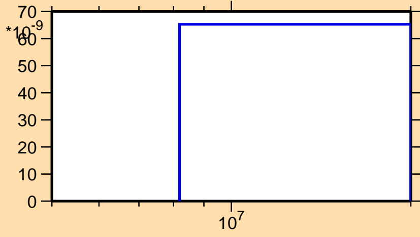
\sigma vs. E for ^{179}\text{Pt}(\text{mt117})
