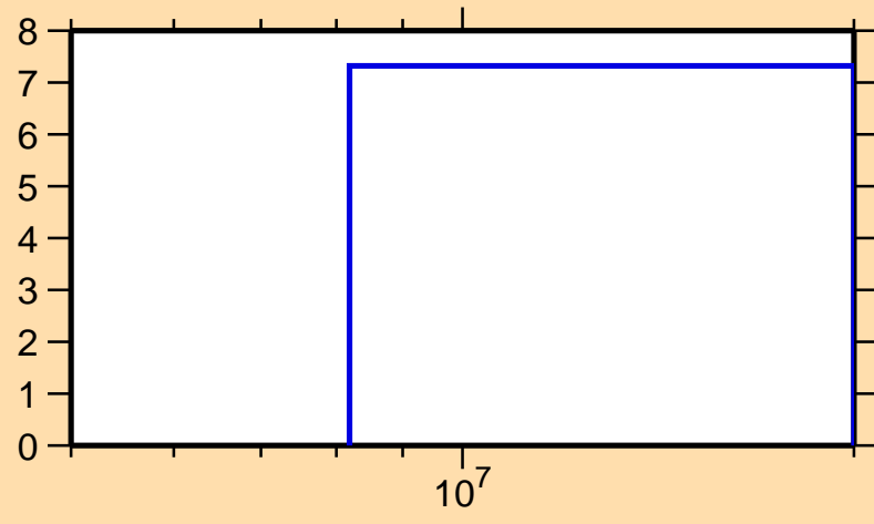
\Delta\sigma/\sigma vs. E for ^{179}\text{Pt}(n,\text{nonel.})
