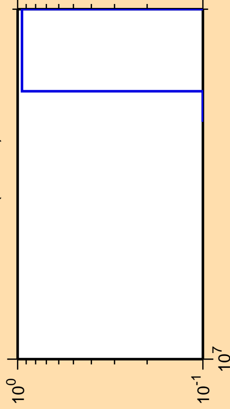
\Delta\sigma/\sigma vs. E for ^{180}\text{Pt}(n,3n\alpha)
