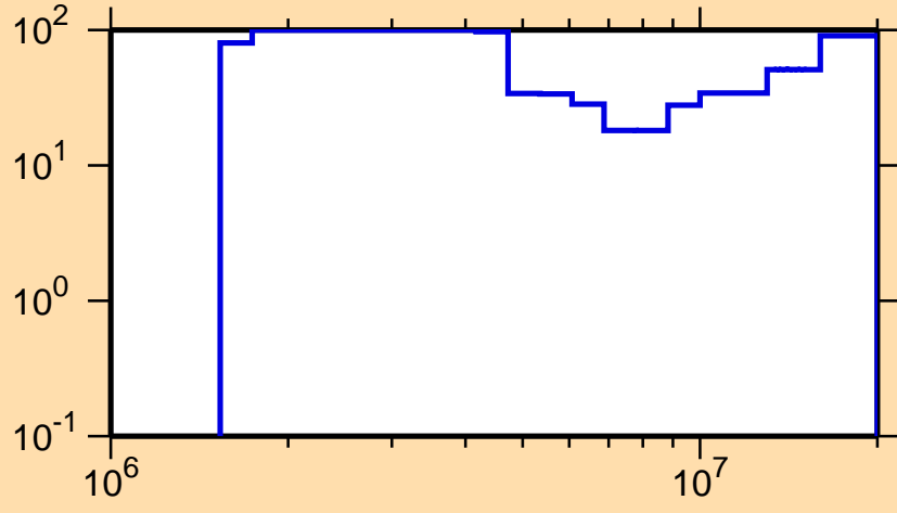
\Delta\sigma/\sigma vs. E for ^{180}\text{Pt}(n,n\text{cont.})
