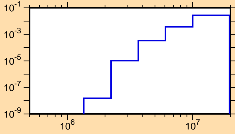
\sigma vs. E for ^{180}\text{Pt}(n,n\alpha)
