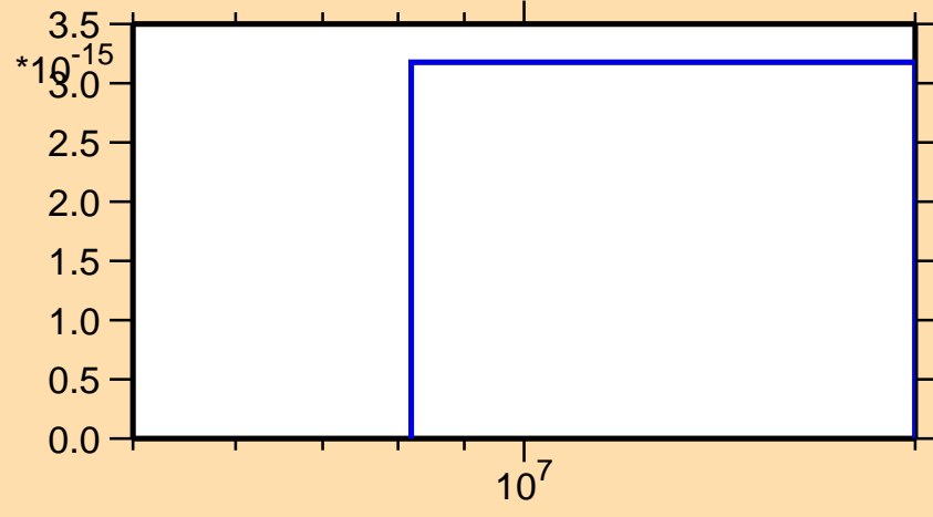
\sigma vs. E for ^{180}\text{Pt}(n,3n\alpha)
