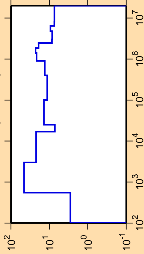
\Delta\sigma/\sigma vs. E for ^{180}\text{Pt}(n,\text{nonel.})
