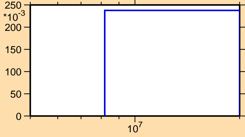
\sigma vs. E for ^{180}\text{Pt}(n,2n)
