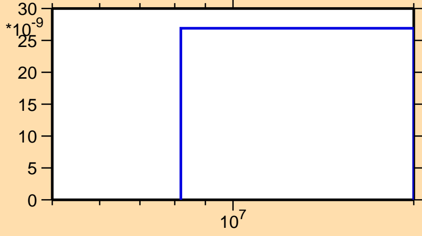
\sigma vs. E for ^{180}\text{Pt}(\text{mt117})
