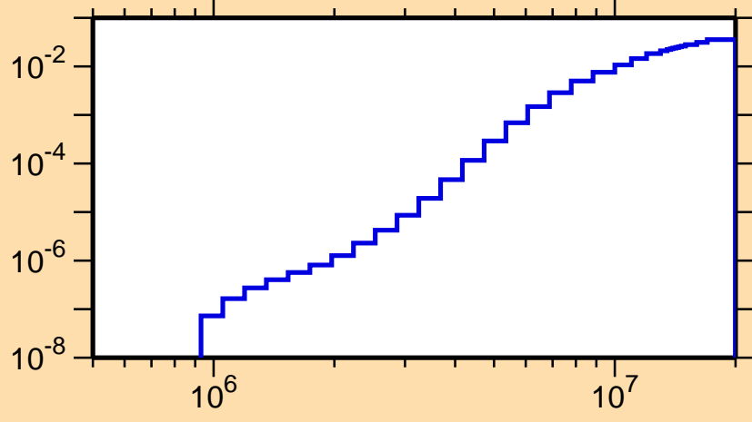
\sigma vs. E for ^{181}\text{Pt}(n,n\alpha)
