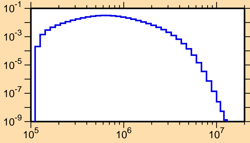
\sigma vs. E for ^{181}\text{Pt}(n,n_3)
