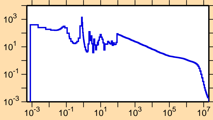
\sigma vs. E for ^{181}\text{Pt}(n,\gamma)
