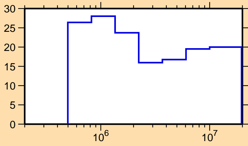
\Delta\sigma/\sigma vs. E for ^{181}\text{Pt}(n,nonel.)
