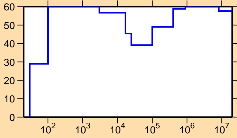
\Delta\sigma/\sigma vs. E for ^{181}\text{Pt}(n,\gamma)
