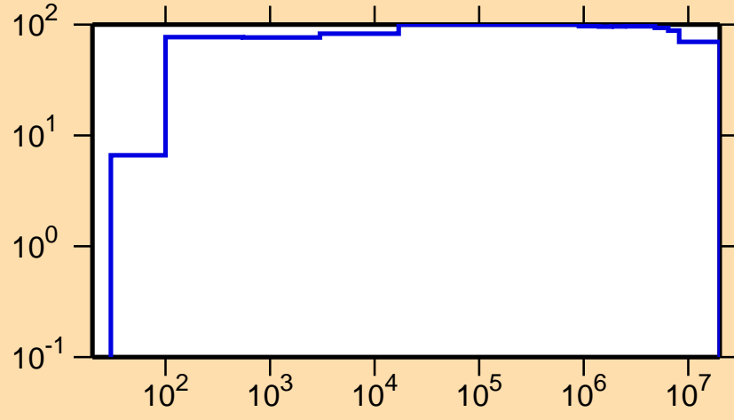
\Delta\sigma/\sigma vs. E for ^{181}\text{Pt}(n,p)
