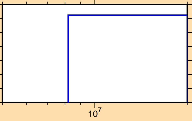
\sigma vs. E for ^{181}\text{Pt}(n,2n\alpha)
