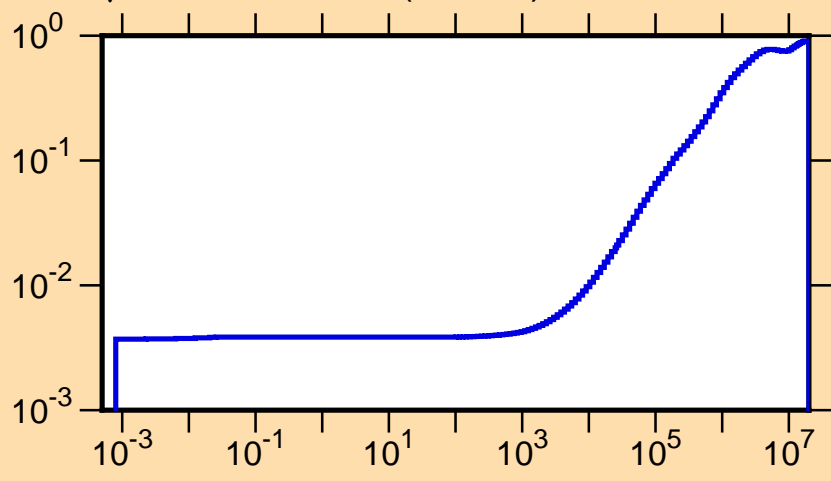
\mu vs. E for ^{182}\text{Pt}(\text{mt251})
