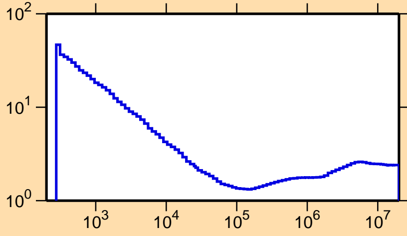
\sigma vs. E for ^{182}\text{Pt}(n,\text{nonel.})
