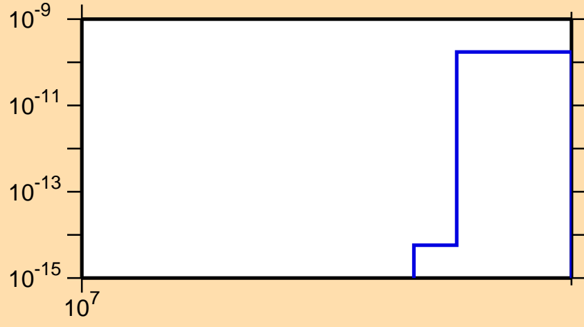
\sigma vs. E for ^{182}\text{Pt}(n,nt)
