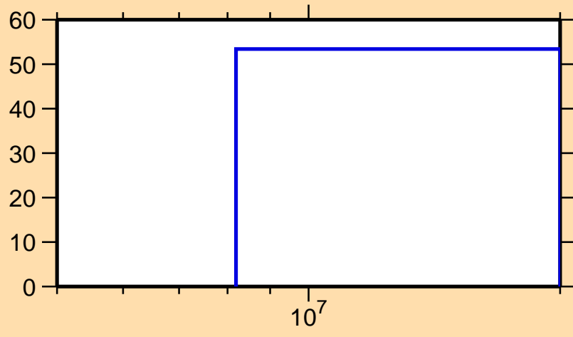
\Delta\sigma/\sigma vs. E for ^{182}\text{Pt}(n, 2n)
