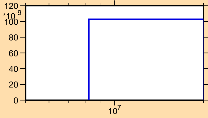
\sigma vs. E for ^{182}\text{Pt}(n,\text{He3})
