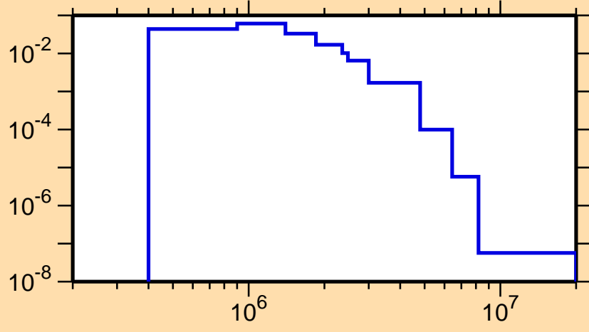
\sigma vs. E for ^{182}\text{Pt}(n,n_3)
