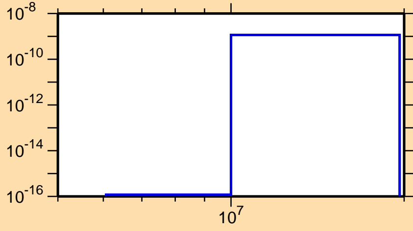
\sigma vs. E for ^{183}\text{Pt}(\text{mt117})
