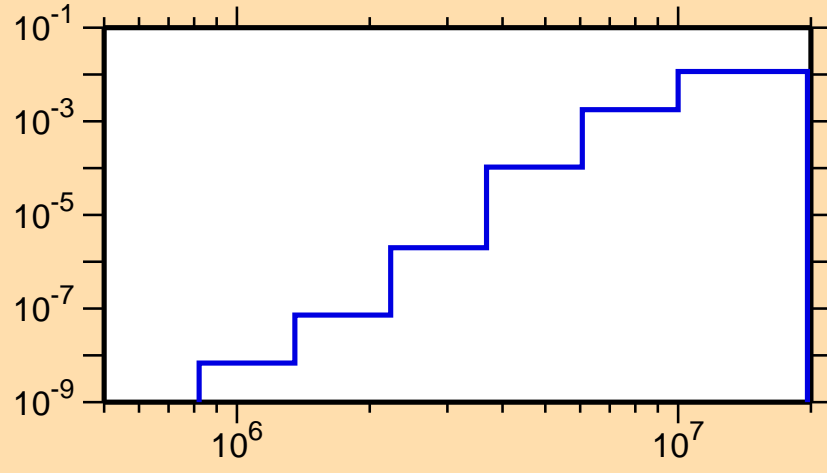
\sigma vs. E for ^{183}\text{Pt}(n,n\alpha)
