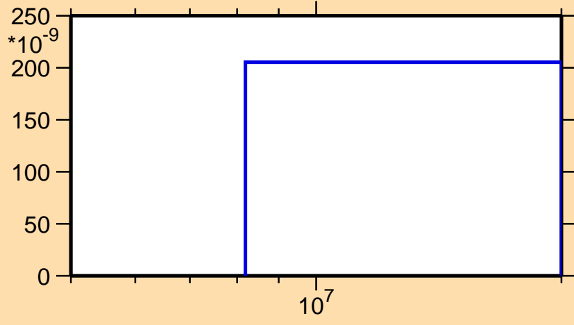
\sigma vs. E for ^{183}\text{Pt}(n,\text{He3})
