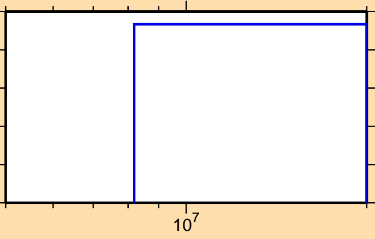
\sigma vs. E for ^{183}\text{Pt}(\text{mt117})
