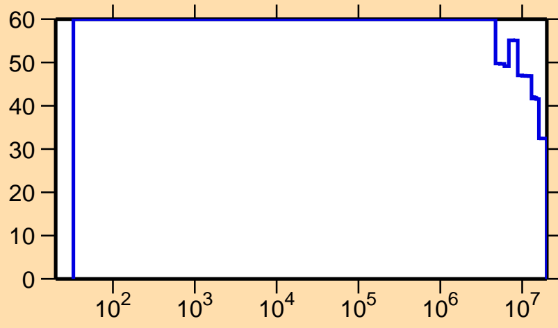
\Delta\sigma/\sigma vs. E for ^{183}\text{Pt}(n,p)
