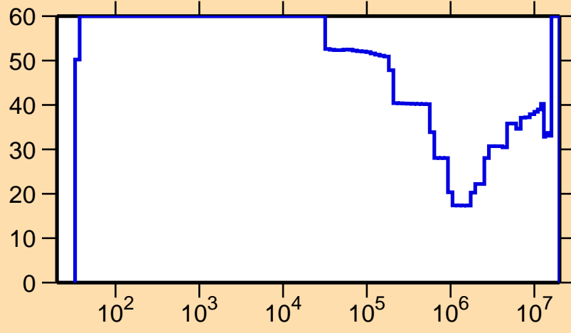
\Delta\sigma/\sigma vs. E for ^{183}\text{Pt}(n,\gamma)
