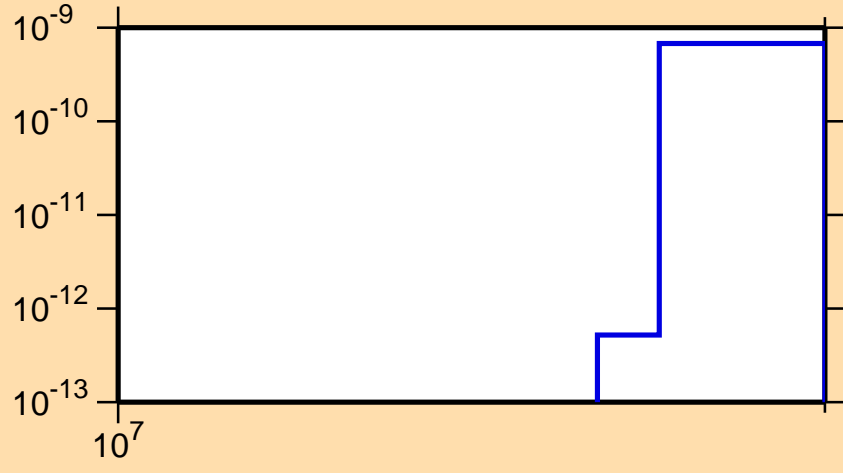
\sigma vs. E for ^{183}\text{Pt}(n,3n\alpha)
