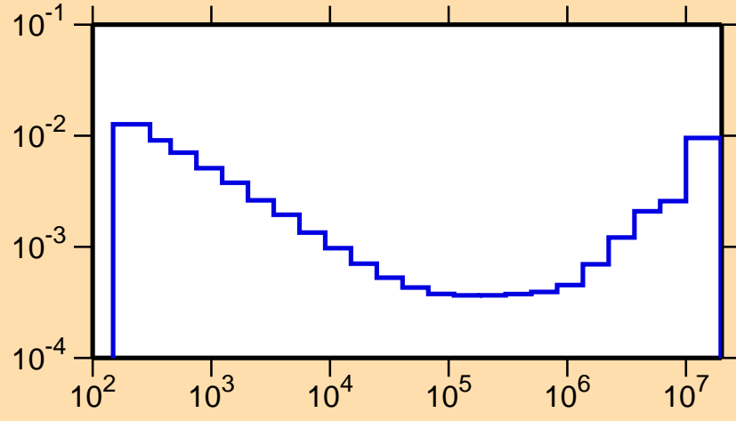
\sigma vs. E for ^{184}\text{Pt}(n,\alpha)
