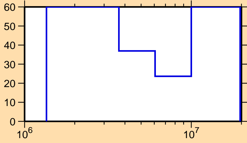
\Delta\sigma/\sigma vs. E for ^{184}\text{Pt}(n,n\text{cont.})
