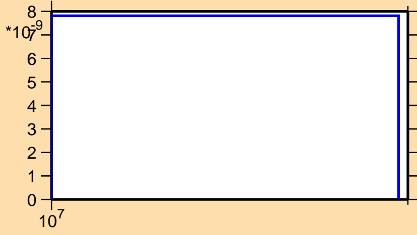
\sigma vs. E for ^{184}\text{Pt}(n,3n\alpha)
