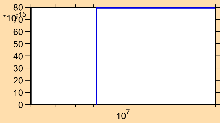
\sigma vs. E for ^{184}\text{Pt}(n,\text{pt})
