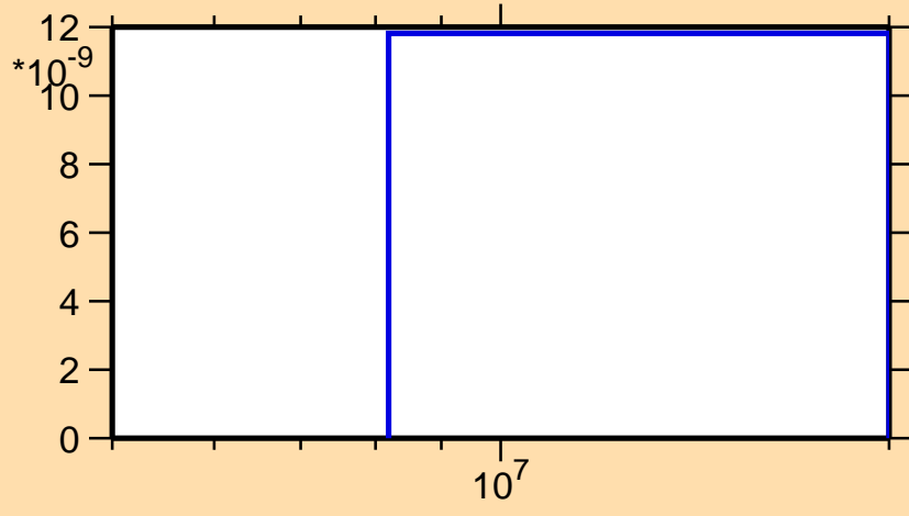
\sigma vs. E for ^{184}\text{Pt}(\text{mt } 45)
