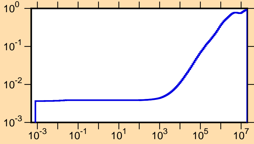
\mu vs. E for ^{185}\text{Pt}(\text{mt251})
