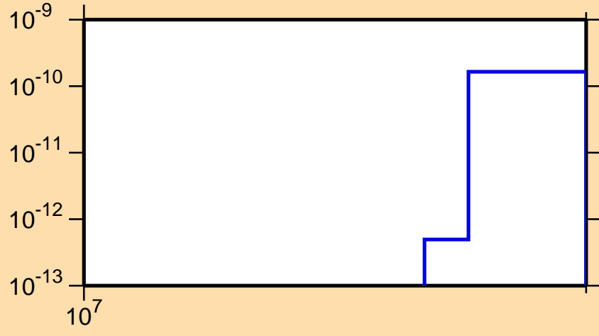
\sigma vs. E for ^{185}\text{Pt}(n,3n\alpha)
