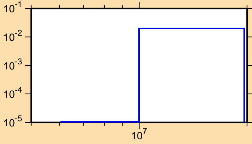
\sigma vs. E for ^{185}\text{Pt}(n,2n\alpha)
