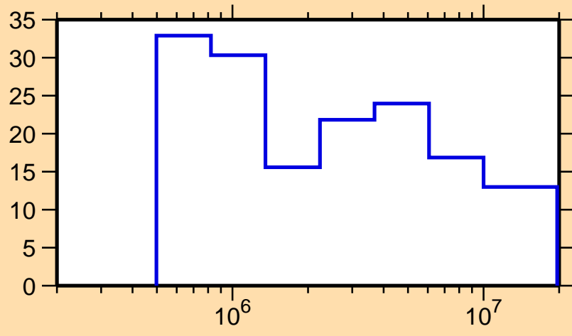
\Delta\sigma/\sigma vs. E for ^{185}\text{Pt}(n, el.)
