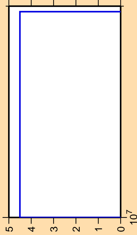
\Delta\sigma/\sigma vs. E for ^{185}\text{Pt}(n,3n\alpha)
