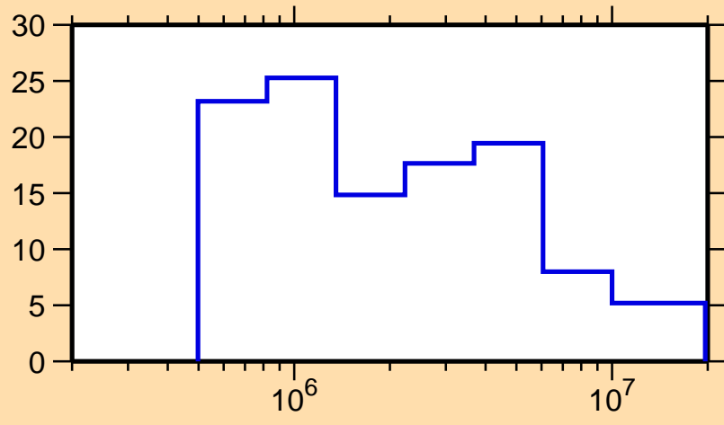
\Delta\sigma/\sigma vs. E for ^{185}\text{Pt}(n, tot.)
