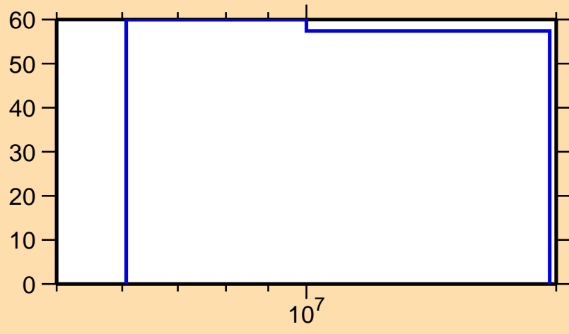
\Delta\sigma/\sigma vs. E for ^{185}\text{Pt}(n,2n)
