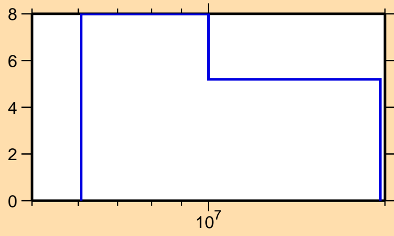
\Delta\sigma/\sigma vs. E for ^{185}\text{Pt}(n,\text{tot.})
