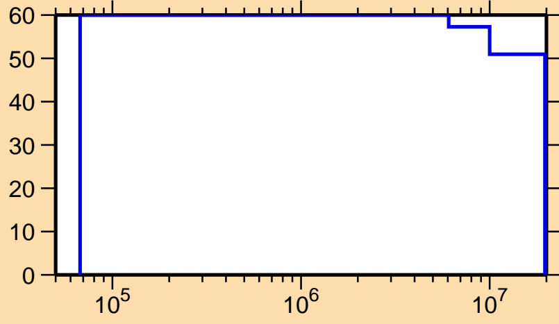
\Delta\sigma/\sigma vs. E for ^{185}\text{Pt}(n,n_1)
