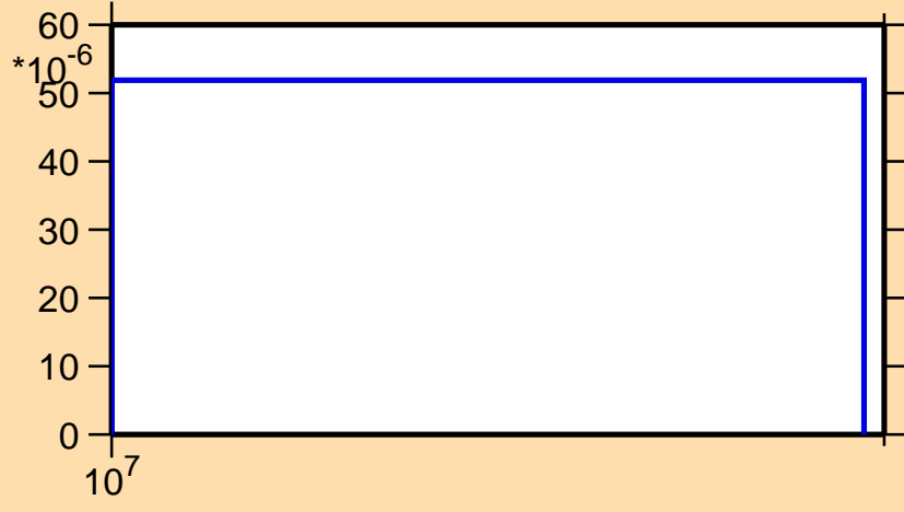
\sigma vs. E for ^{185}\text{Pt}(n,3n)
