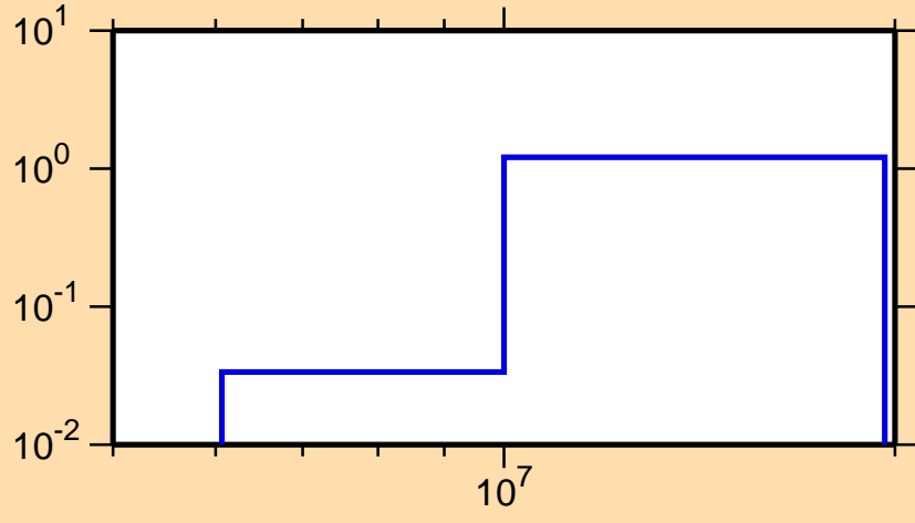
\sigma vs. E for ^{185}\text{Pt}(n,2n)
