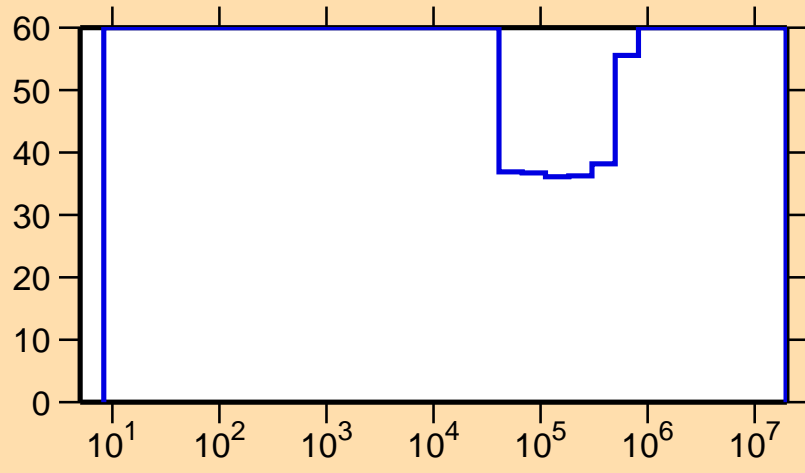
\Delta\sigma/\sigma vs. E for ^{185}\text{Pt}(n,\gamma)
