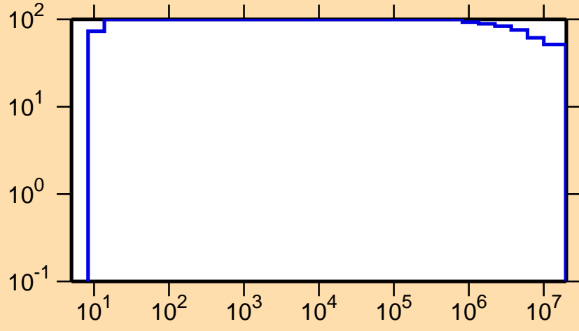
\Delta\sigma/\sigma vs. E for ^{185}\text{Pt}(n,p)
