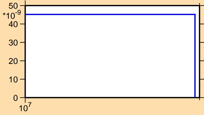
\sigma vs. E for ^{185}\text{Pt}(n,\text{nd})
