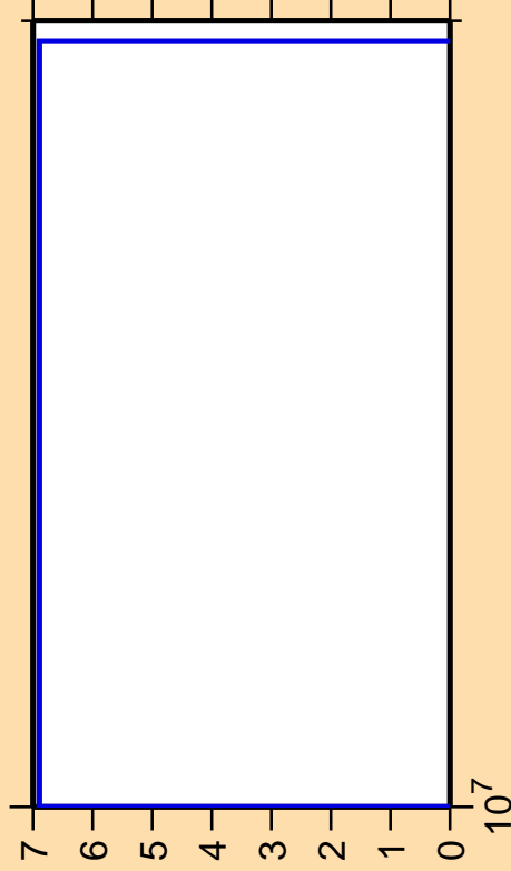
\Delta\sigma/\sigma vs. E for ^{185}\text{Pt}(\text{mt } 34)
