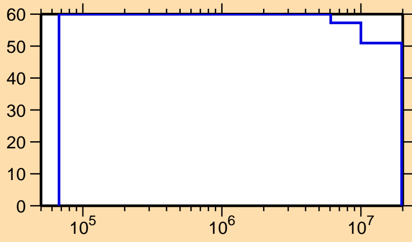
\Delta\sigma/\sigma vs. E for ^{185}\text{Pt}(n,n_1)
