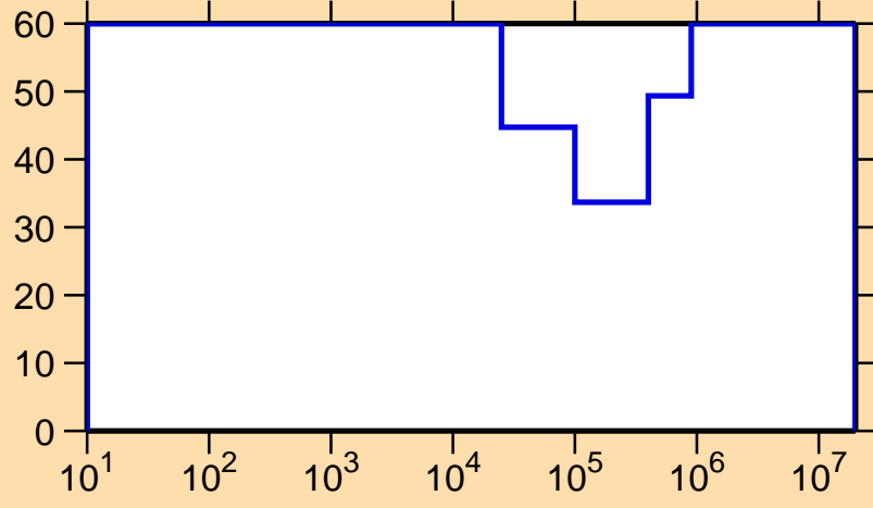
\Delta\sigma/\sigma vs. E for ^{185}\text{Pt}(n,\gamma)
