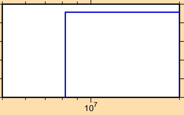
\sigma vs. E for ^{185}\text{Pt}(n,3n)
