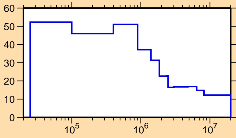
\Delta\sigma/\sigma vs. E for ^{185}\text{Pt}(n,\text{nonel.})
