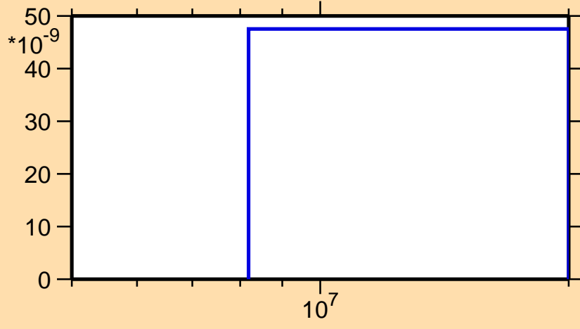
\sigma vs. E for ^{185}\text{Pt}(n,\text{He3})
