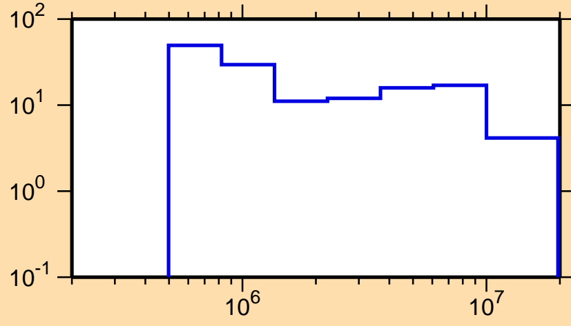
\Delta\sigma/\sigma vs. E for ^{185}\text{Pt}(n,tot.)
