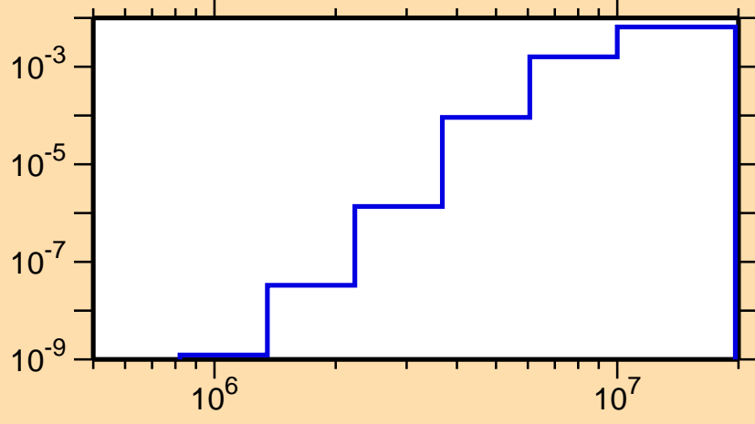
\sigma vs. E for ^{185}\text{Pt}(n,n\alpha)
