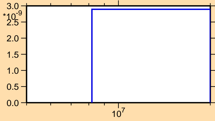
\sigma vs. E for ^{185}\text{Pt}(\text{mt } 45)
