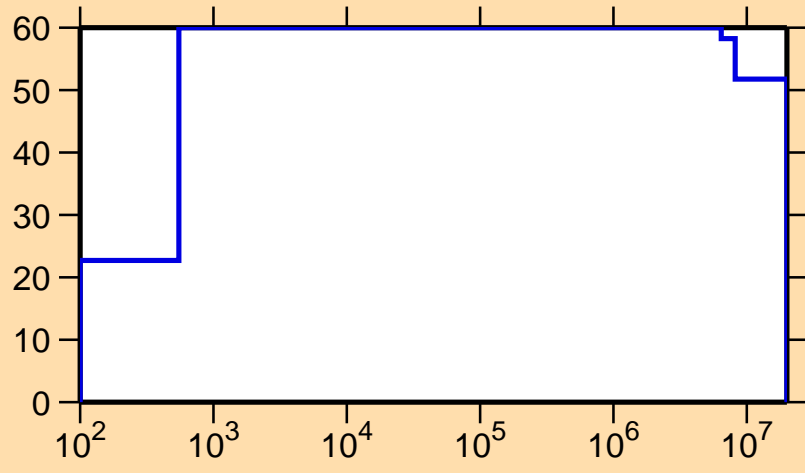
\Delta\sigma/\sigma vs. E for ^{185}\text{Pt}(n,p)
