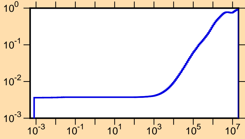
\mu vs. E for ^{186}\text{Pt}(\text{mt251})
