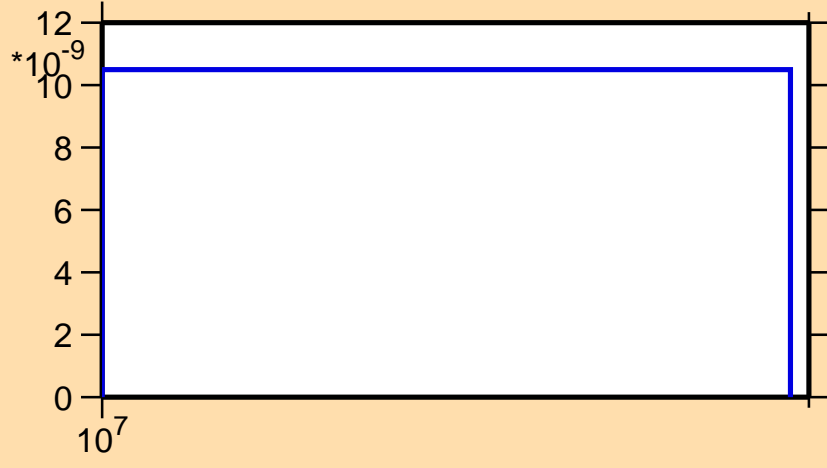
\sigma vs. E for ^{186}\text{Pt}(n,3n\alpha)
