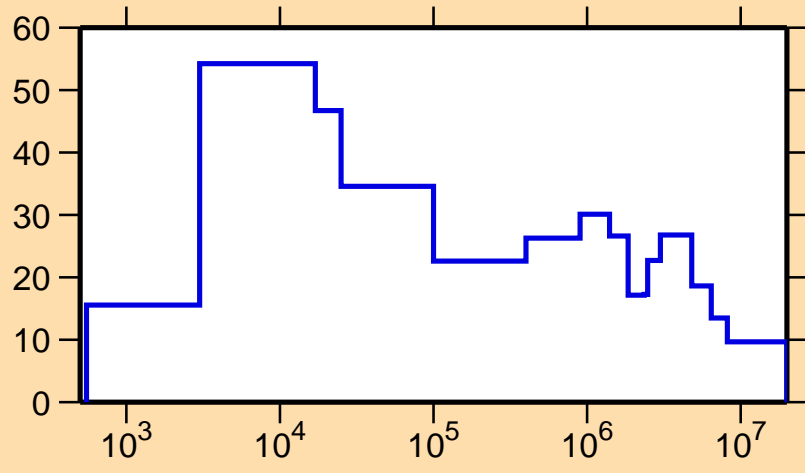
\Delta\sigma/\sigma vs. E for ^{186}\text{Pt}(n,el.)
