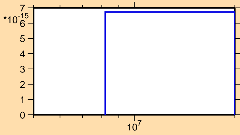
\sigma vs. E for ^{186}\text{Pt}(n,\text{pt})
