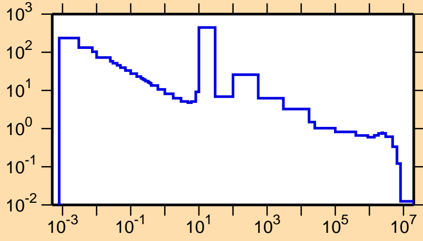
\sigma vs. E for ^{186}\text{Pt}(n,\gamma)
