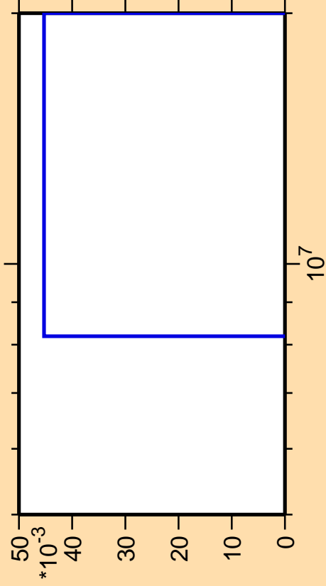
\Delta\sigma/\sigma vs. E for ^{186}\text{Pt}(n,\text{pt})
