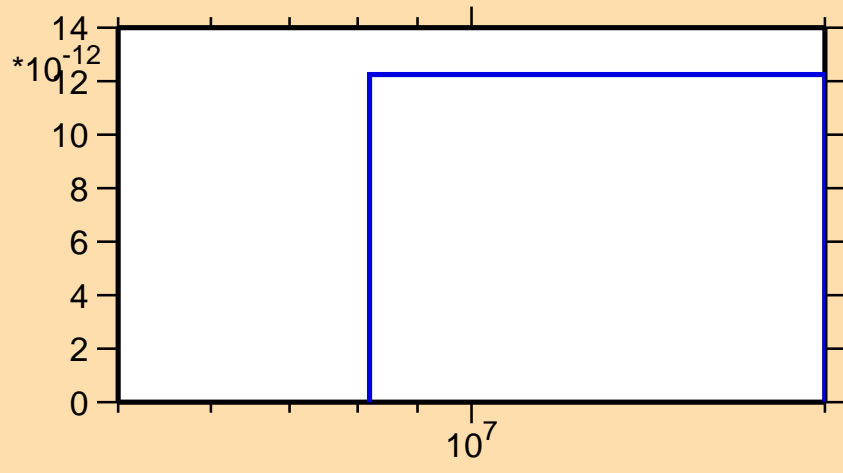
\sigma vs. E for ^{186}\text{Pt}(n,nt)
