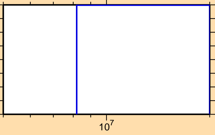
\sigma vs. E for ^{186}\text{Pt}(n,2np)
