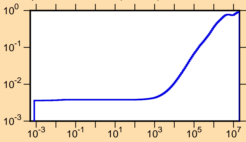
\mu vs. E for ^{187}\text{Pt}(\text{mt251})
