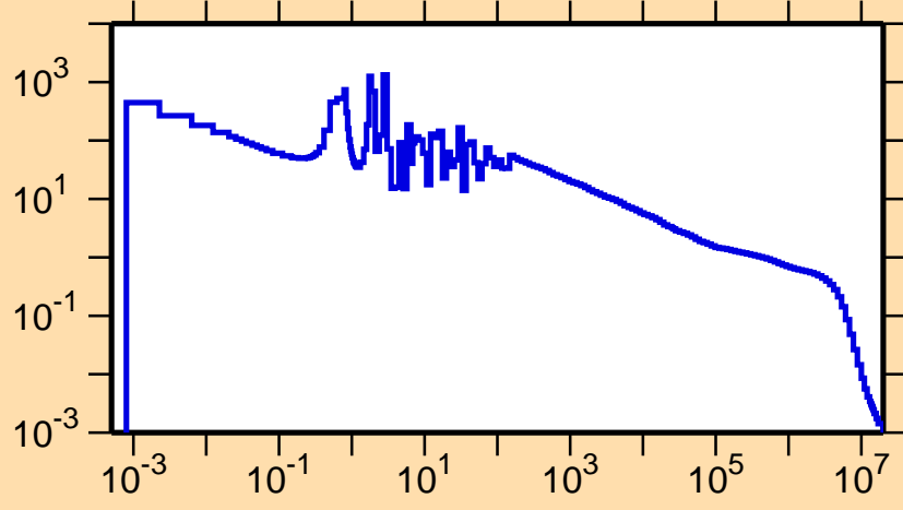
\sigma vs. E for ^{187}\text{Pt}(n,\gamma)
