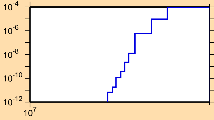
\sigma vs. E for ^{187}\text{Pt}(n,2np)
