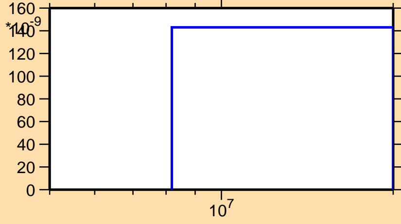
\sigma vs. E for ^{187}\text{Pt}(n,\text{nd})
