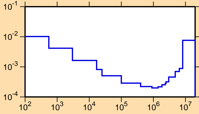
\sigma vs. E for ^{187}\text{Pt}(n,\alpha)
