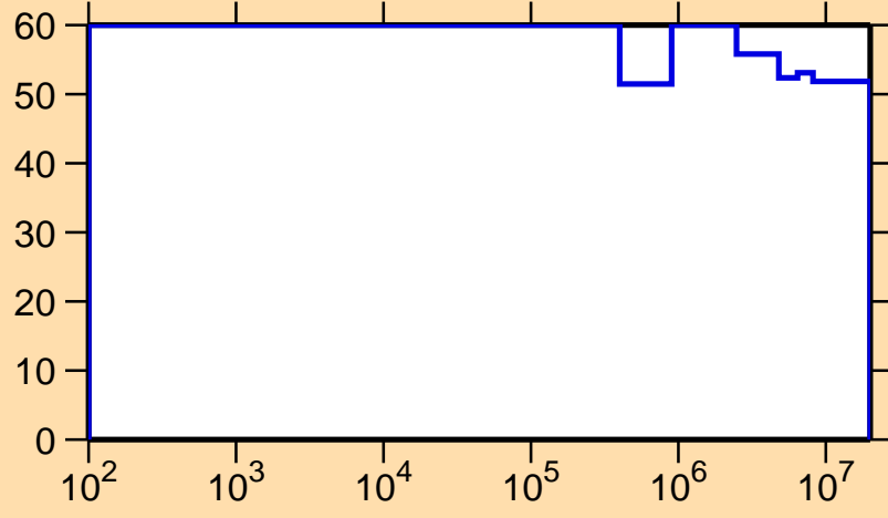
\Delta\sigma/\sigma vs. E for ^{187}\text{Pt}(n,p)
