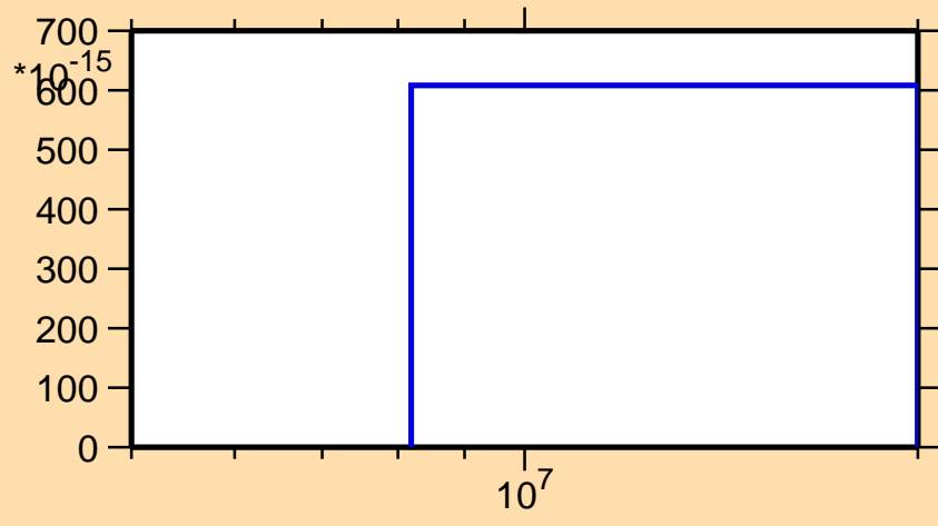
\sigma vs. E for ^{187}\text{Pt}(\text{mt } 34)
