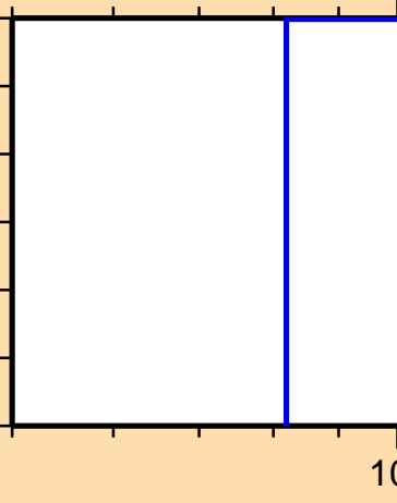
\sigma vs. E for ^{188}\text{Pt}(\text{mt117})
