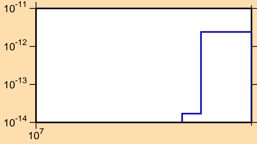
\sigma vs. E for ^{189}\text{Pt}(n,\text{pt})
