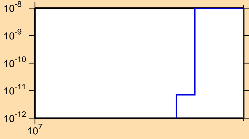
\sigma vs. E for ^{189}\text{Pt}(n,nt)
