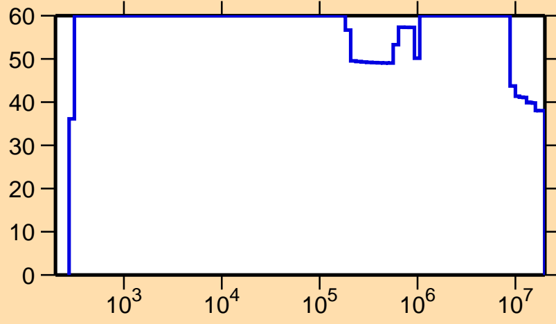
\Delta\sigma/\sigma vs. E for ^{189}\text{Pt}(n,p)
