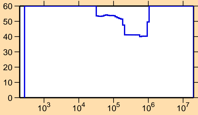
\Delta\sigma/\sigma vs. E for ^{189}\text{Pt}(n,\gamma)
