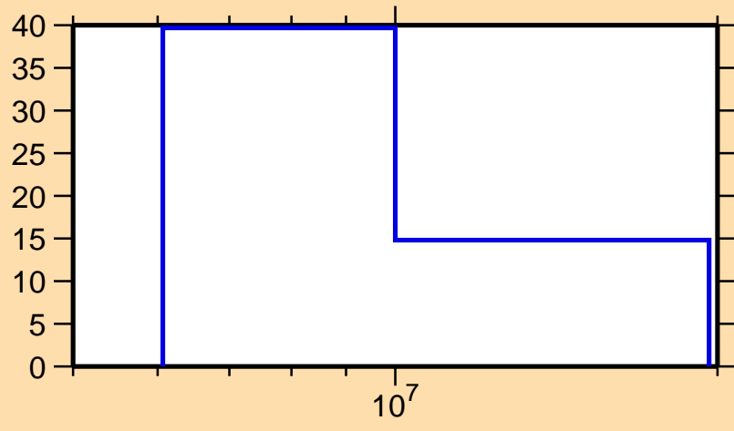
\Delta\sigma/\sigma vs. E for ^{189}\text{Pt}(n,2n)
