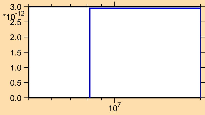
\sigma vs. E for ^{189}\text{Pt}(\text{mt117})
