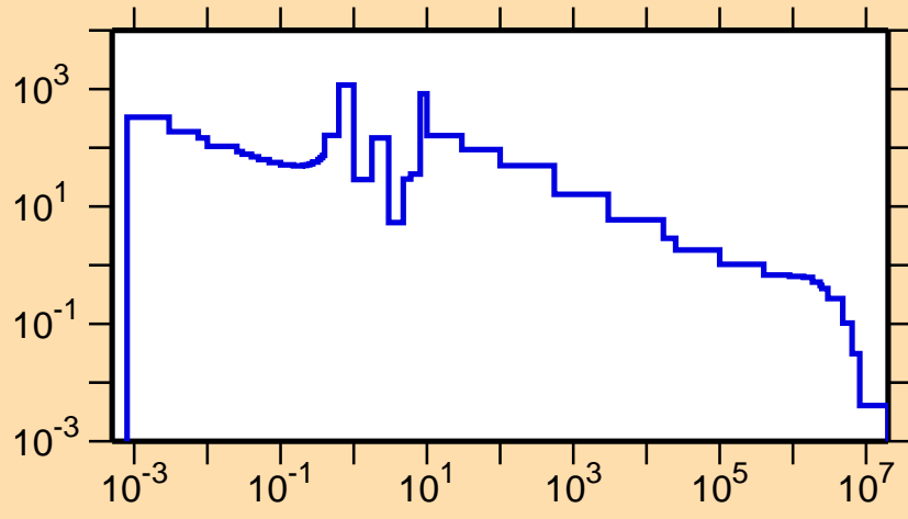
\sigma vs. E for ^{189}\text{Pt}(n,\gamma)
