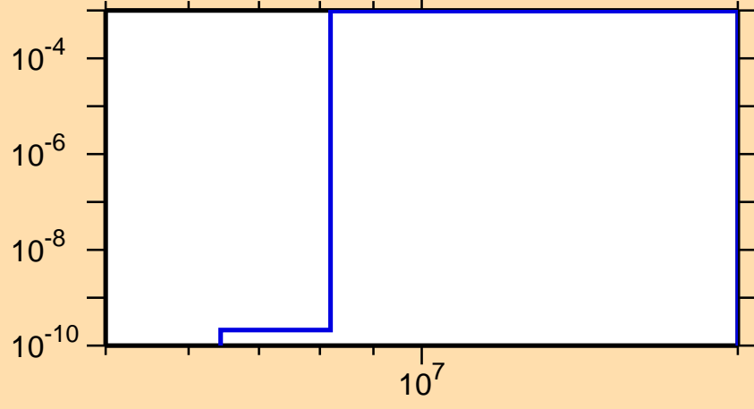
\sigma vs. E for ^{189}\text{Pt}(n,d)
