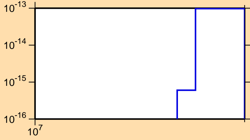
\sigma vs. E for ^{190}\text{Pt}(n,\text{pd})
