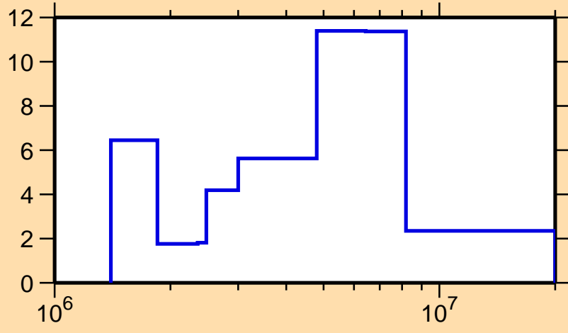
\Delta\sigma/\sigma vs. E for ^{190}\text{Pt}(n,\text{tot.})
