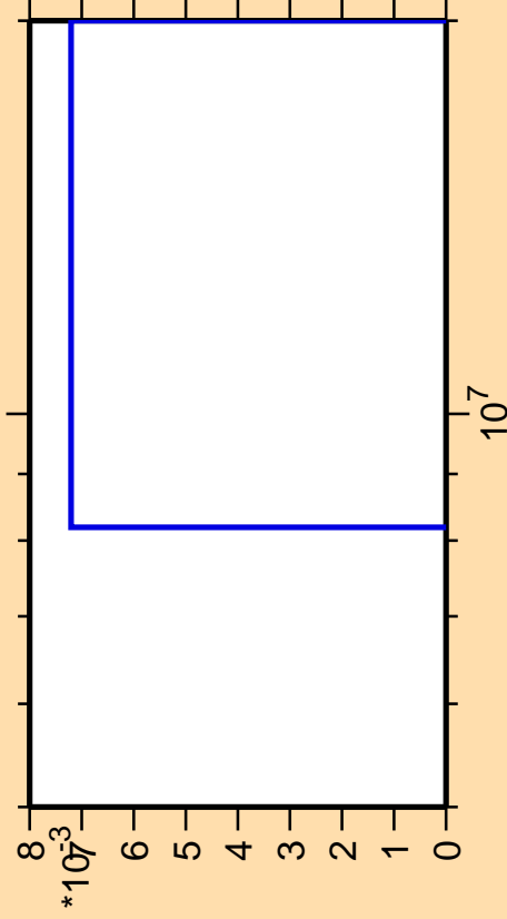
\Delta\sigma/\sigma vs. E for ^{190}\text{Pt}(n,\text{pd})
