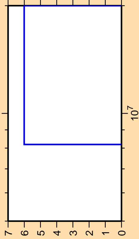
\Delta\sigma/\sigma vs. E for ^{190}\text{Pt}(n,n\text{cont.})
