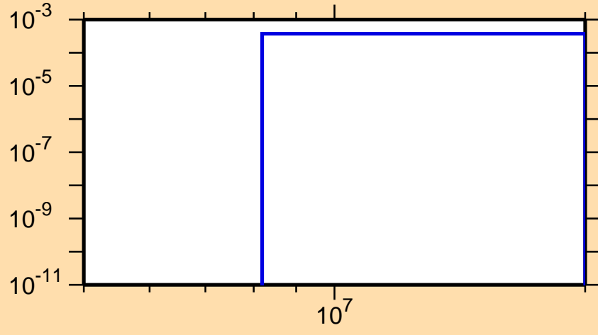
\sigma vs. E for ^{190}\text{Pt}(n,np)
