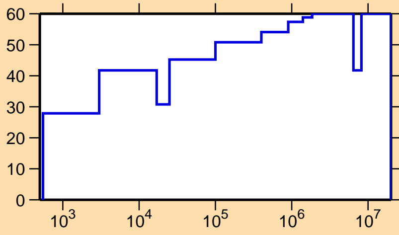
\Delta\sigma/\sigma vs. E for ^{190}\text{Pt}(n,\gamma)
