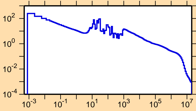
\sigma vs. E for ^{191}\text{Pt}(n,\gamma)
