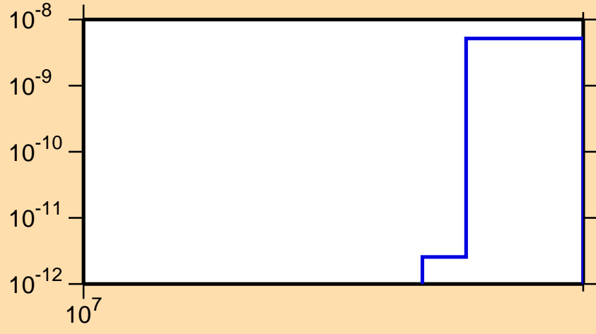
\sigma vs. E for ^{191}\text{Pt}(n,nt)
