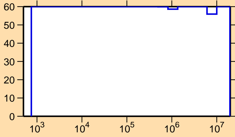
\Delta\sigma/\sigma vs. E for ^{191}\text{Pt}(n,\gamma)
