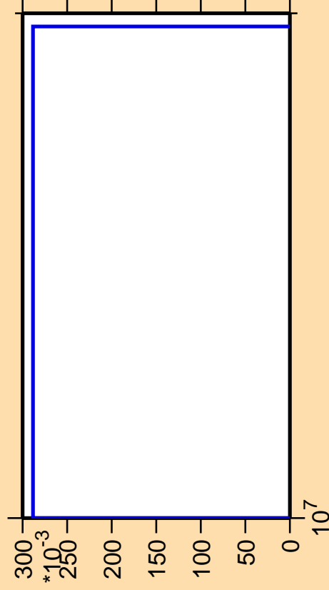
\Delta\sigma/\sigma vs. E for ^{191}\text{Pt}(\text{mt117})
