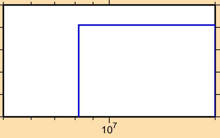
\sigma vs. E for ^{191}\text{Pt}(n,3n)
