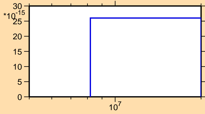
\sigma vs. E for ^{191}\text{Pt}(\text{mt } 45)
