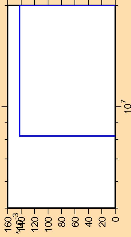
\Delta\sigma/\sigma vs. E for ^{191}\text{Pt}(\text{mt } 45)
