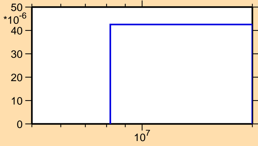
\sigma vs. E for ^{191}\text{Pt}(n,t)
