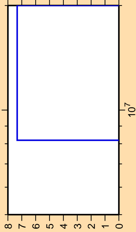
\Delta\sigma/\sigma vs. E for ^{191}\text{Pt}(n,3n\alpha)
