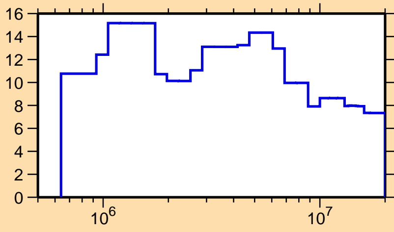
\Delta\sigma/\sigma vs. E for ^{193}\text{Pt}(n, el.)
