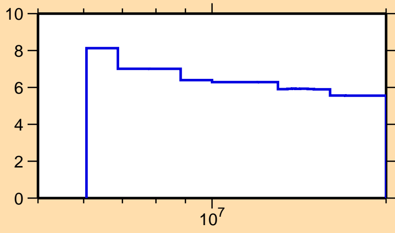
\Delta\sigma/\sigma vs. E for ^{193}\text{Pt}(n,\text{nonel.})
