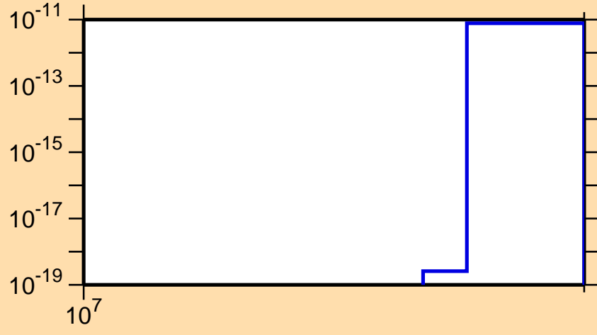
\sigma vs. E for ^{193}\text{Pt}(n,3n\alpha)
