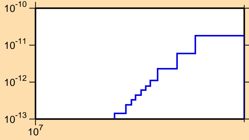
\sigma vs. E for ^{193}\text{Pt}(n,p\alpha)
