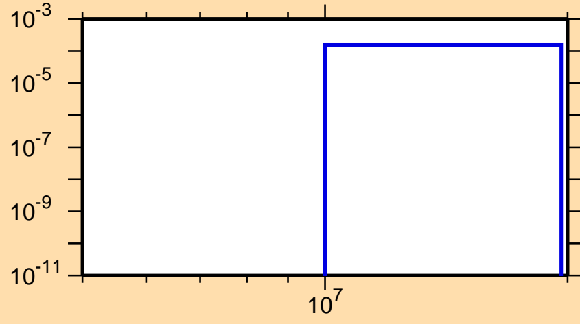
\sigma vs. E for ^{193}\text{Pt}(n,np)
