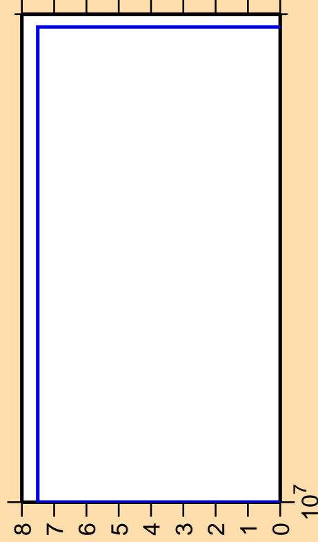
\Delta\sigma/\sigma vs. E for ^{193}\text{Pt}(n,p\alpha)
