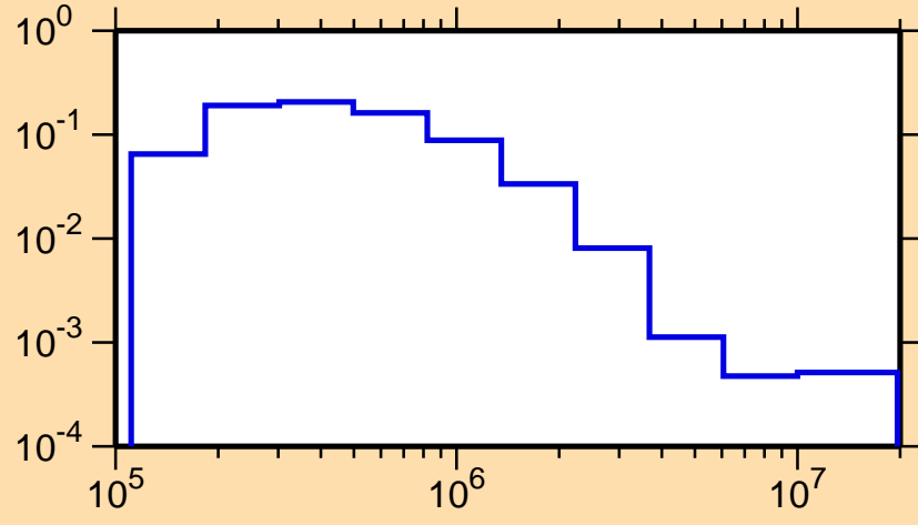
\sigma vs. E for ^{193}\text{Pt}(n,n_3)
