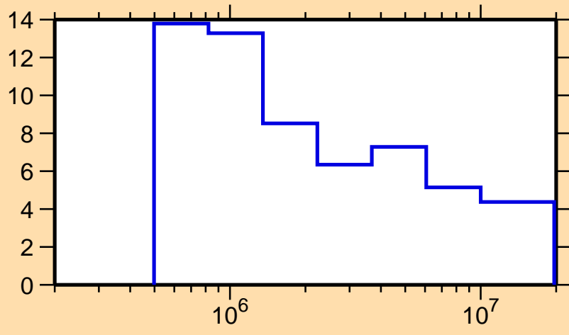
\Delta\sigma/\sigma vs. E for ^{193}\text{Pt}(n, \text{tot.})
