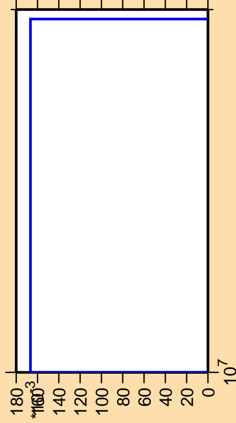
\Delta\sigma/\sigma vs. E for ^{193}\text{Pt}(n,3n\alpha)
