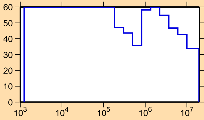
\Delta\sigma/\sigma vs. E for ^{193}\text{Pt}(n,n_1)
