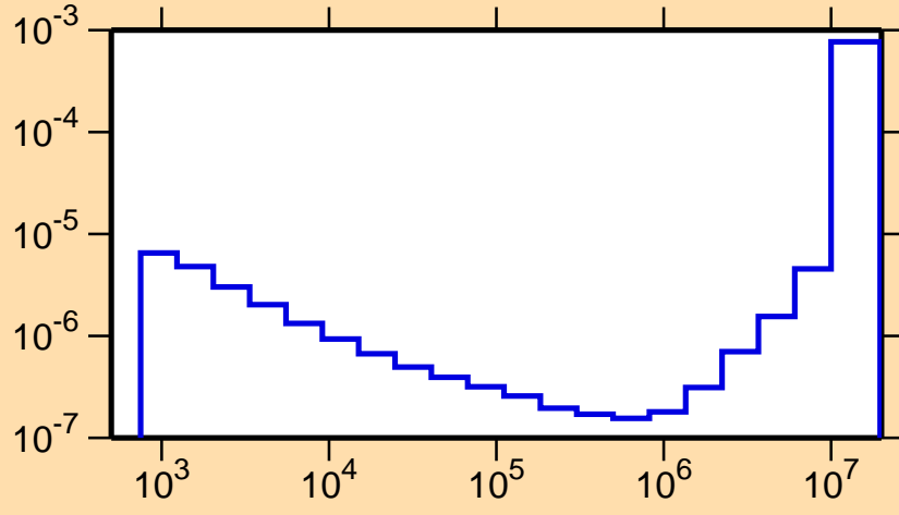
\sigma vs. E for ^{193}\text{Pt}(n,\alpha)
