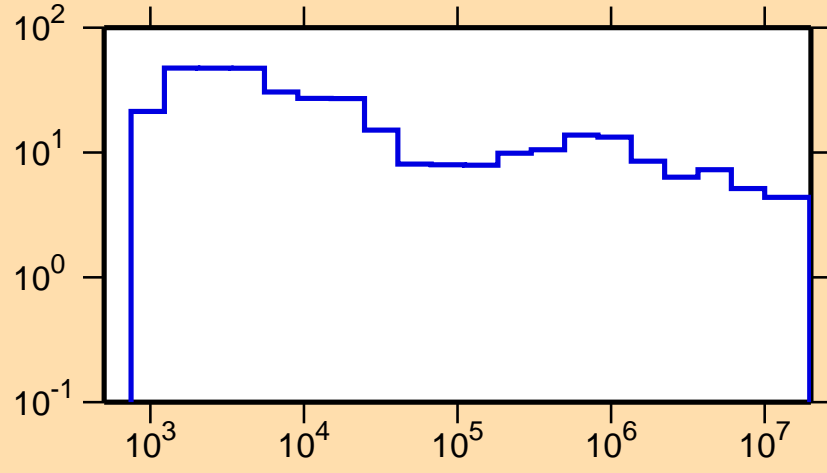
\Delta\sigma/\sigma vs. E for ^{193}\text{Pt}(n,\text{tot.})
