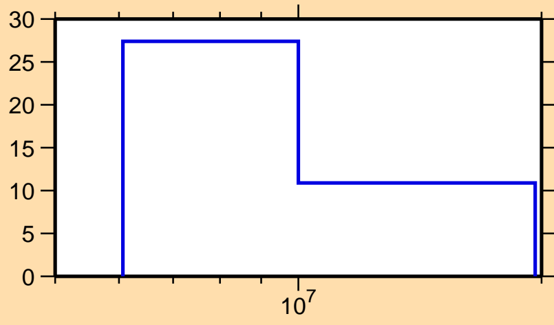
\Delta\sigma/\sigma vs. E for ^{193}\text{Pt}(n,2n)
