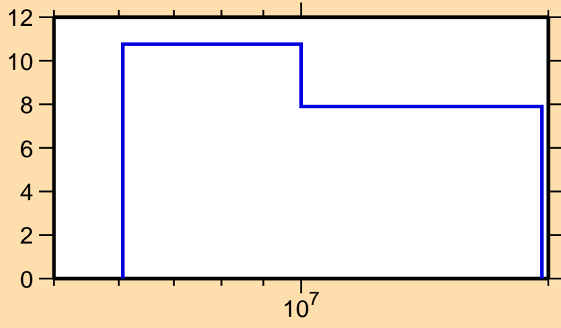
\Delta\sigma/\sigma vs. E for ^{193}\text{Pt}(n,\text{el.})
