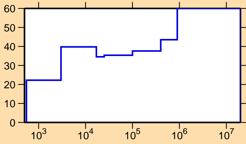
\Delta\sigma/\sigma vs. E for ^{193}\text{Pt}(n,\gamma)
