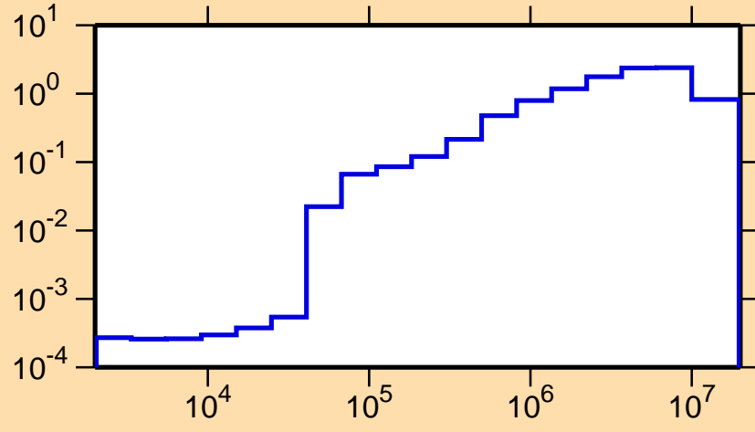
\sigma vs. E for ^{193}\text{Pt}(n,\text{inel.})
