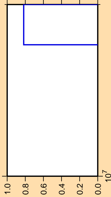
\Delta\sigma/\sigma vs. E for ^{194}\text{Pt}(n,p\alpha)
