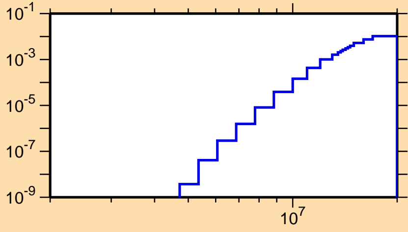
\sigma vs. E for ^{194}\text{Pt}(n,p)
