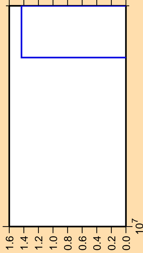
\Delta\sigma/\sigma vs. E for ^{194}\text{Pt}(n,3n\alpha)
